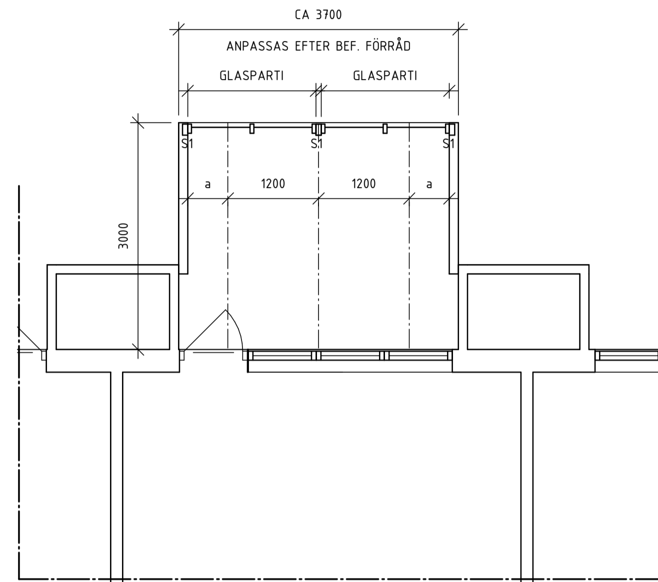
PLAN
