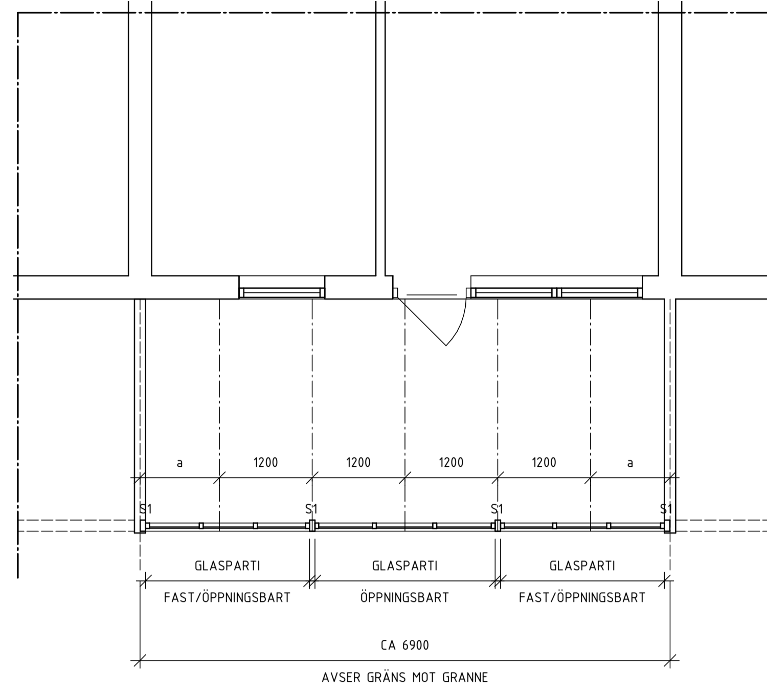
PLAN
